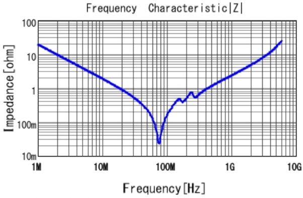
GCM2195C1H822JA16 |Z| DCOV, 25degC
