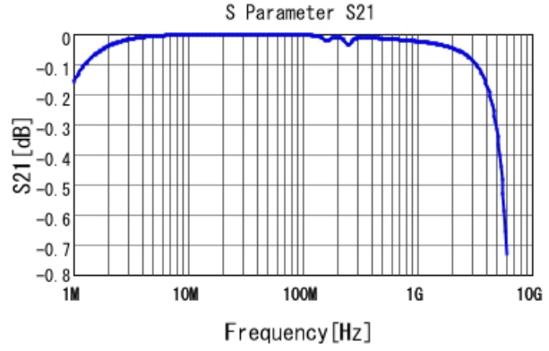
GCM2195C1H822JA16 S21 DCOV, 25degC
