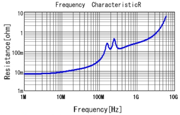
GCM2195C1H822JA16 R DCOV, 25degC
