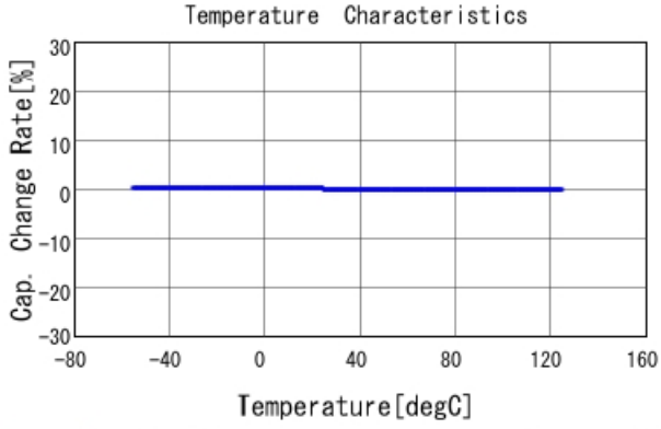
GCM2195C1H822JA16 C-Temp. capchange, DCOV, AC1Vrms
