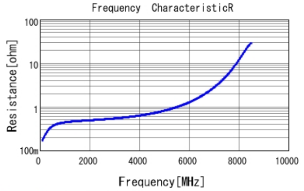
GRM1885C1H2R9BA01 R DCOV, 25degC
