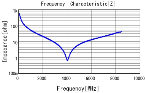
GRM1885C1H2R9BA01 |Z| DCOV, 25degC
