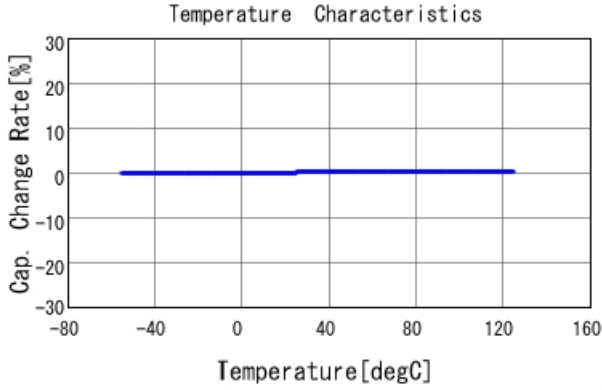
GRM1885C1H2R9BA01 C-Temp. capchange, DCOV, AC1Vrms
