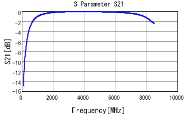
GRM1885C1H2R9BA01 S21 DCOV, 25degC
