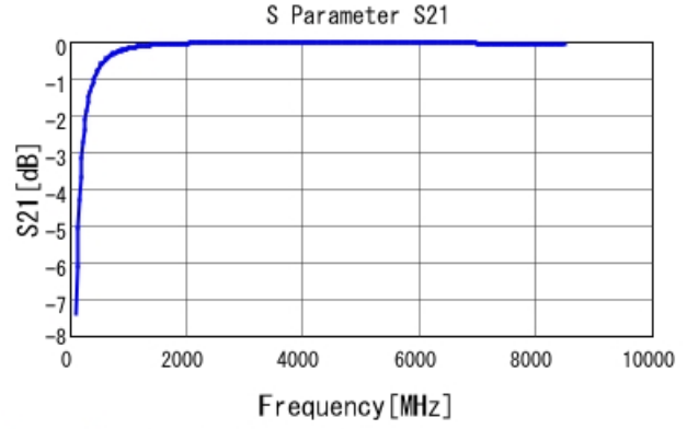
GRM0225C1E7R5BA03 S21 DC0V, 25degC
