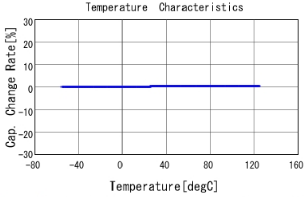
GRM0225C1E7R5BA03 C-Temp. capchange, DC0V, AC1Vrms
