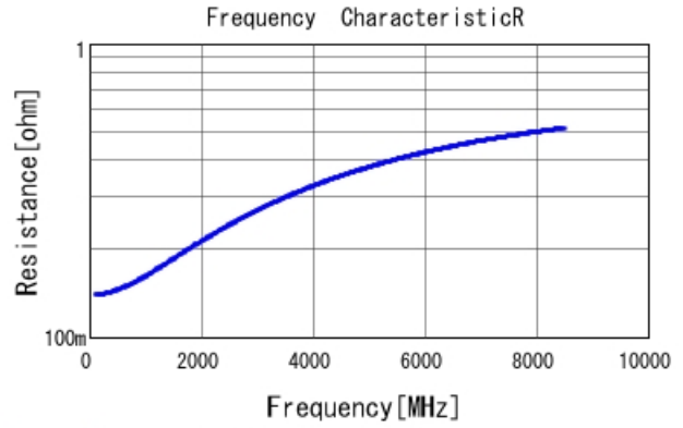
GRM0225C1E7R5BA03 R DCOV, 25degC
