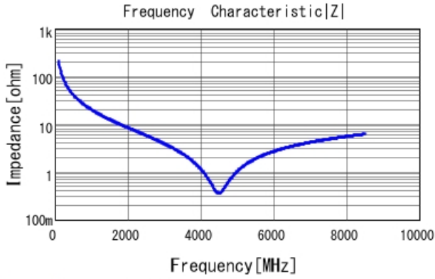
GRM0225C1E7R5BA03 |Z| DCOV, 25degC
