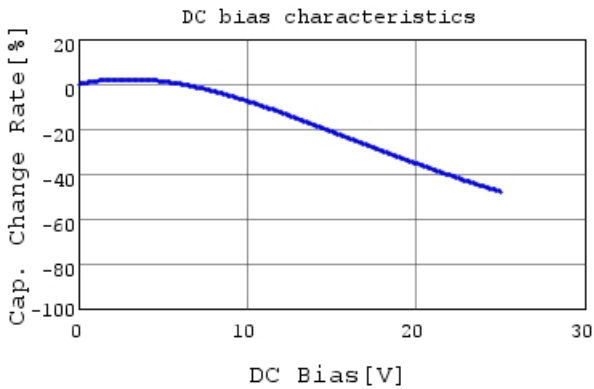
KRM55QR71E336KH01 C-DC bias capchange, 25.0c
