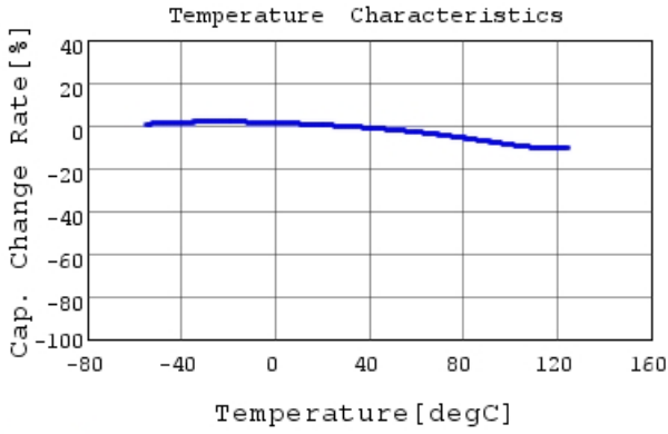
KRM55QR71E336KH01 C-Temp. capchange, DCOV, 1
