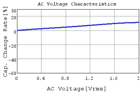
KRM55QR71E336KH01 C-AC Voltage capchange, Dc
