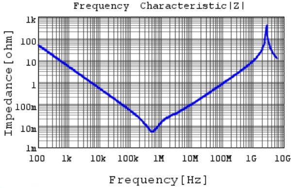
KRM55QR71E336KH01 |Z| DCOV, 25degC
