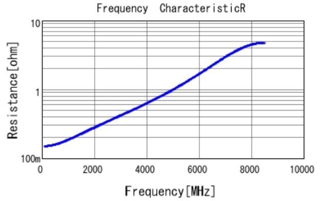
GCM0335C1H270JA16 R DC0V, 25degC
