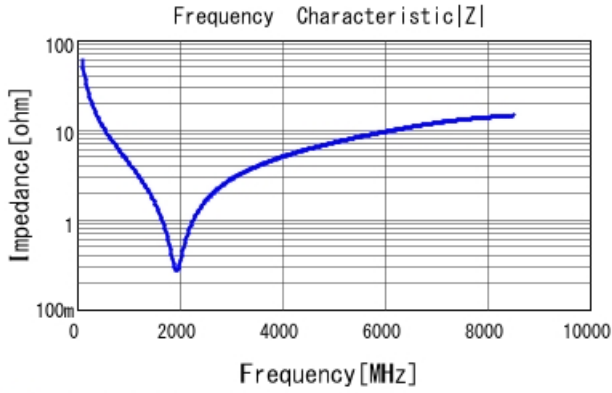
GCM0335C1H270JA16 |Z| DC0V, 25degC
