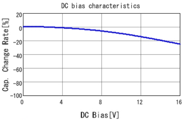
GCJ21BR71C684MA01 C-DC bias capchange, 25.0degC, A
