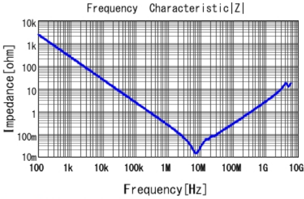
GCJ21BR71C684MA01 |Z| DCOV, 25degC
