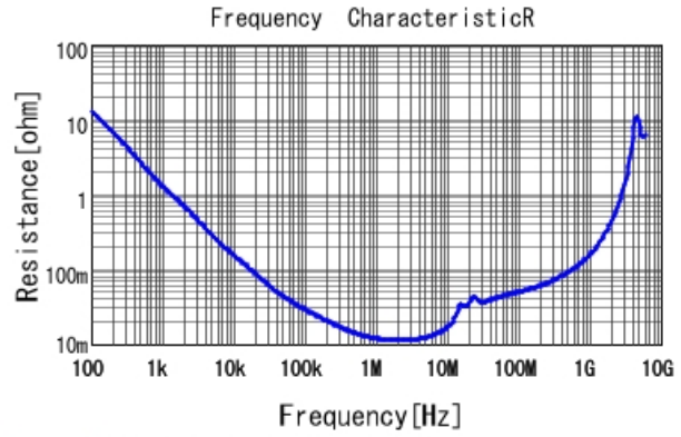
GCJ21BR71C684MA01 R DCOV, 25degC
