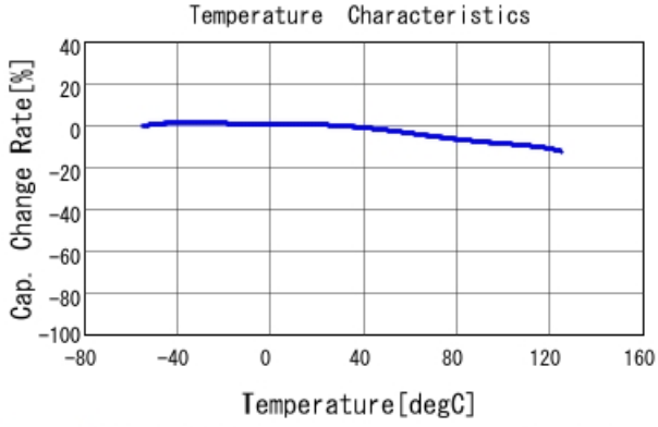
GCJ21BR71C684MA01 C-Temp. capchange, DC0.0V, AC1.C
