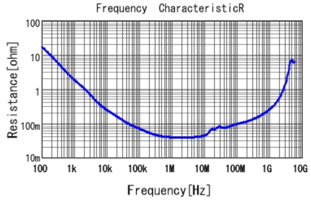
GCJ31ML8YA474MA01 R DCOV, 25degC
