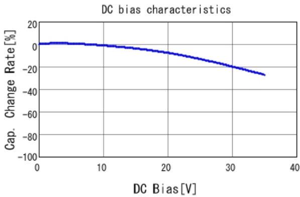
GCJ31ML8YA474MA01 C-DC bias capchange, 25.0degC, A
