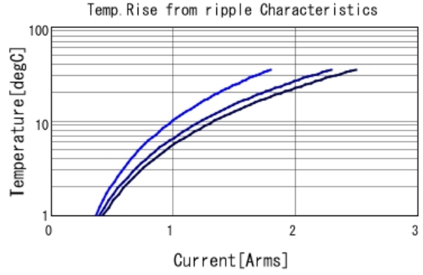
GCJ31ML8YA474MA01 Temp. rise — 200kHz — 500
