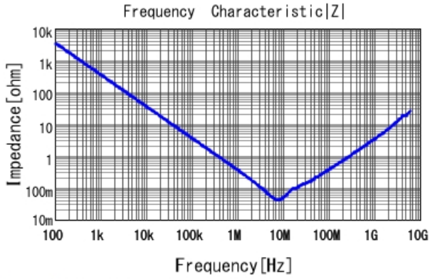
GCJ31ML8YA474MA01 |Z| DCOV, 25degC
