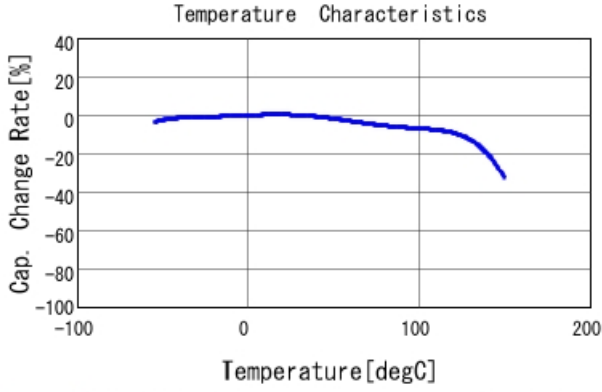
GCJ31ML8YA474MA01 C-Temp. capchange, DC0.0V, AC1.C
