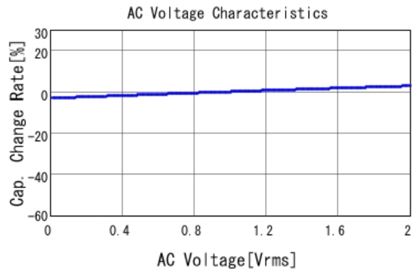
GCJ31ML8YA474MA01 C-AC Voltage capchange, DCOV, 25
