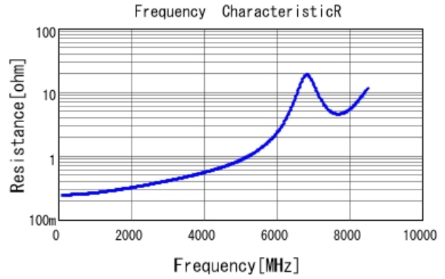
GCM1885C1H4R7BA16 R DCOV, 25degC
