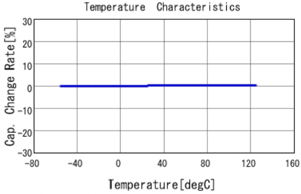
GCM1885C1H4R7BA16 C-Temp. capchange, DCOV, AC1Vrms
