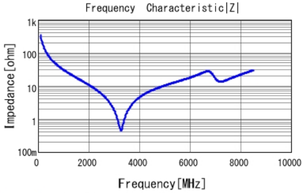
GCM1885C1H4R7BA16 |Z| DCOV, 25degC
