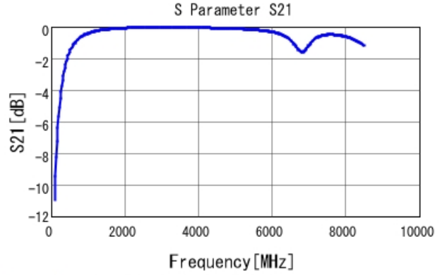
GCM1885C1H4R7BA16 S21 DCOV, 25degC
