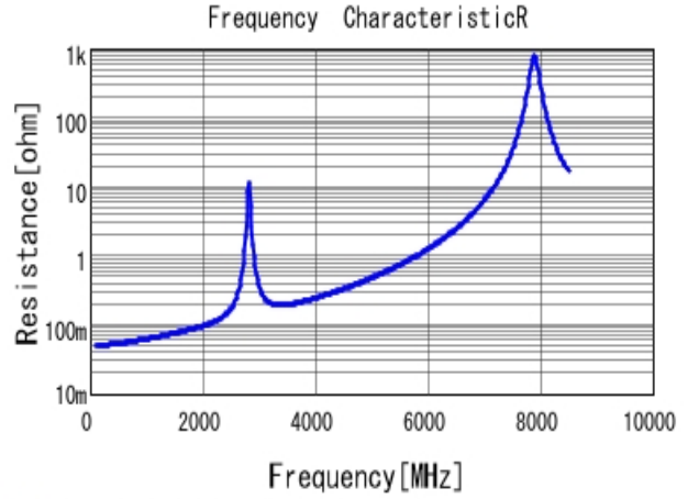
■ GQM2195C1H270GB01 R DC0V, 25degC
