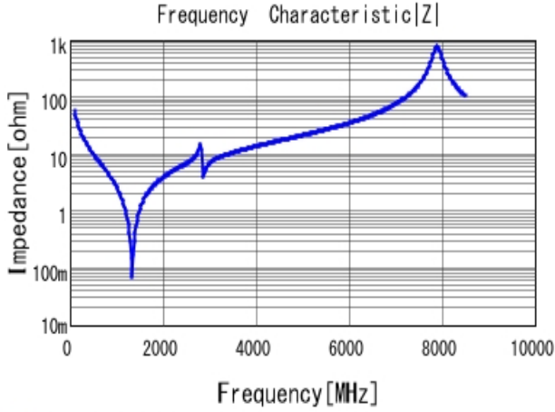
■ GQM2195C1H270GB01 |Z| DC0V, 25degC
