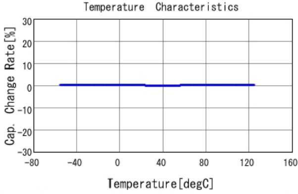
GRM1555C2A7R9DA01 C-Temp. capchange, DCOV, AC1Vrms
