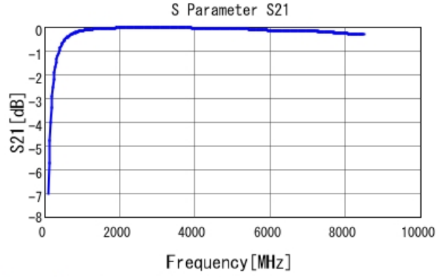
GRM1555C2A7R9DA01 S21 DCOV, 25degC
