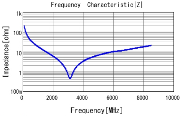
GRM1555C2A7R9DA01 |Z| DCOV, 25degC
