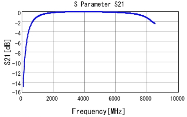
GRM1885C2A2R9CA01 S21 DCOV, 25degC
