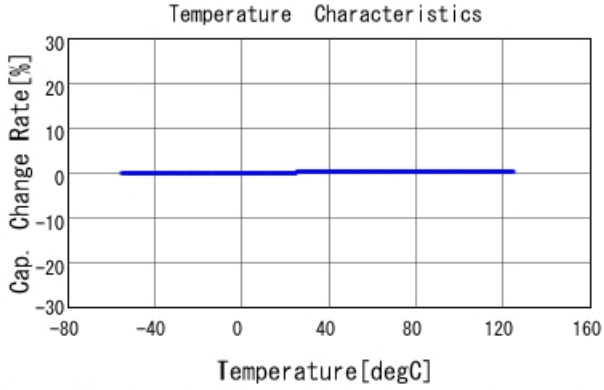
GRM1885C2A2R9CA01 C-Temp. capchange, DCOV, AC1Vrms
