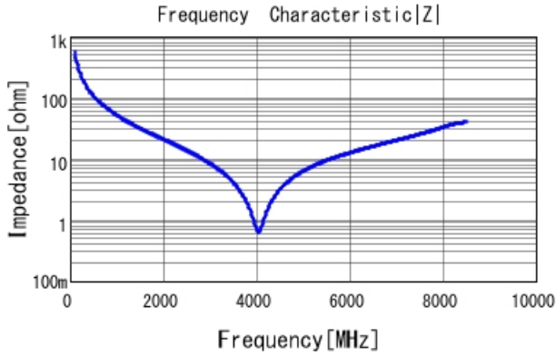
GRM1885C2A2R9CA01 |Z| DCOV, 25degC
