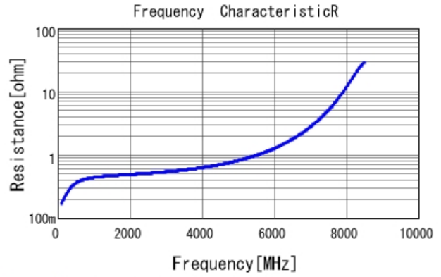
GRM1885C2A2R9CA01 R DCOV, 25degC
