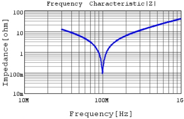
RDE5C1H391J0K1H03B |Z| DCOV, 25degC
