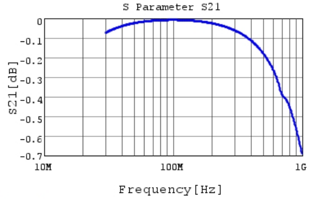
RDE5C1H391J0K1H03B S21 DCOV, 25degC
