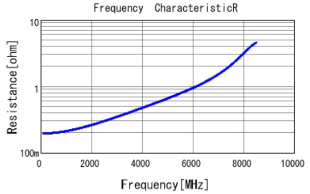
GRM0335C1H6R8BA01 R DCOV, 25degC
