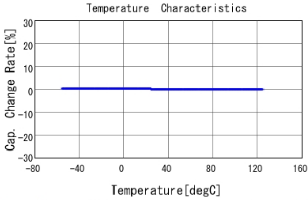
GRM0335C1H6R8BA01 C-Temp. capchange, DCOV, AC1Vrms
