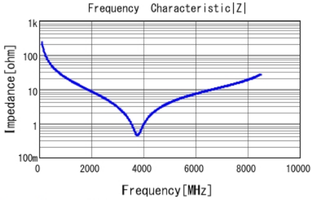
GRM0335C1H6R8BA01 |Z| DCOV, 25degC
