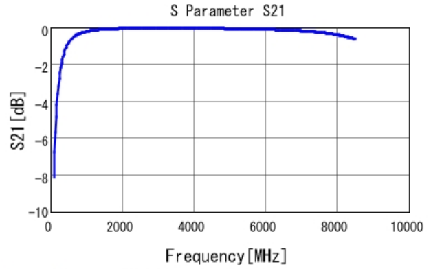
GRM0335C1H6R8BA01 S21 DCOV, 25degC
