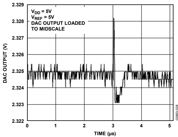
Figure 27. DAC-to-DAC Crosstalk
