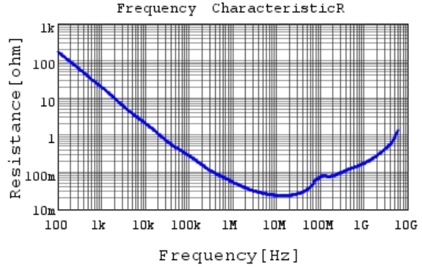
GRM155R71E473MA88 R DCOV, 25degC
