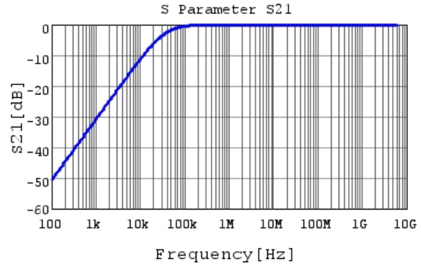
GRM155R71E473MA88 S21 DC0V,25degC
