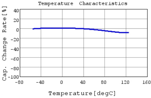
GRM155R71E473MA88 C-Temp. capchange, DC0.0V,
