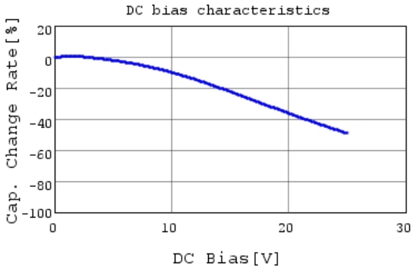
GRM155R71E473MA88 C-DC bias capchange, 25.0c
