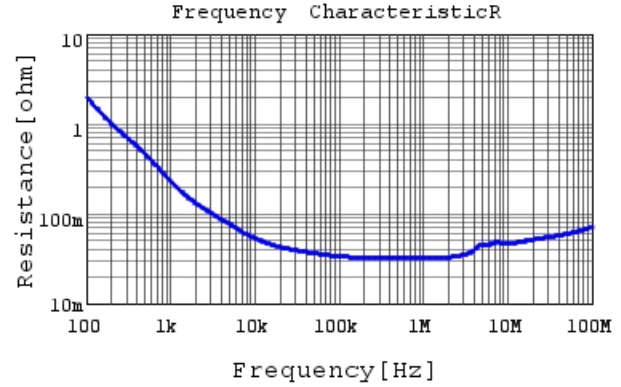
RDEC71E475K2K1H03B R DC0V, 25degC
