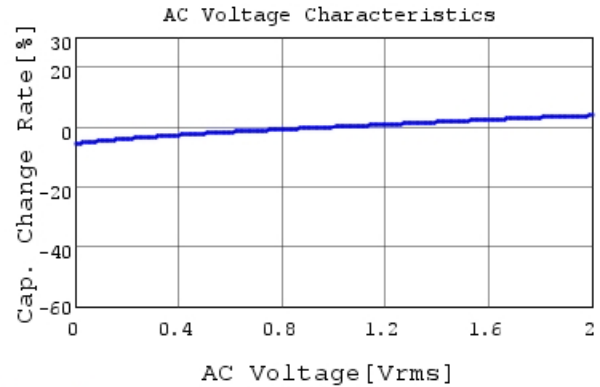
RDEC71E475K2K1H03B C-AC Voltage capchange, I
