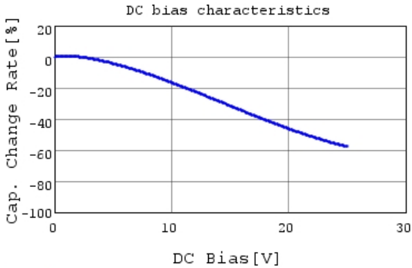
RDEC71E475K2K1H03B C-DC bias capchange, 25.0
