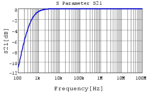
RDEC71E475K2K1H03B S21 DC0V, 25degC
