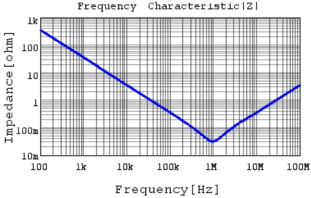
RDEC71E475K2K1H03B |Z| DC0V, 25degC
