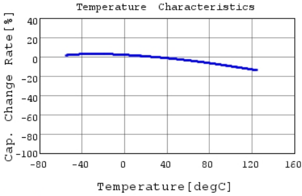
RDEC71E475K2K1H03B C-Temp. capchange, DC0.0V
