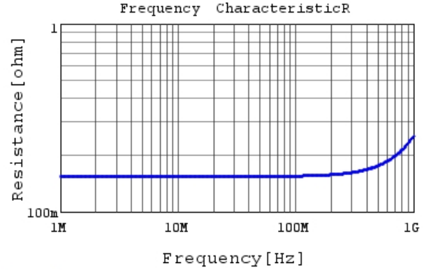
RDE7U3A101J2M1H03A R DCOV, 25degC
