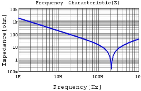
RDE7U3A101J2M1H03A |Z| DCOV, 25degC
