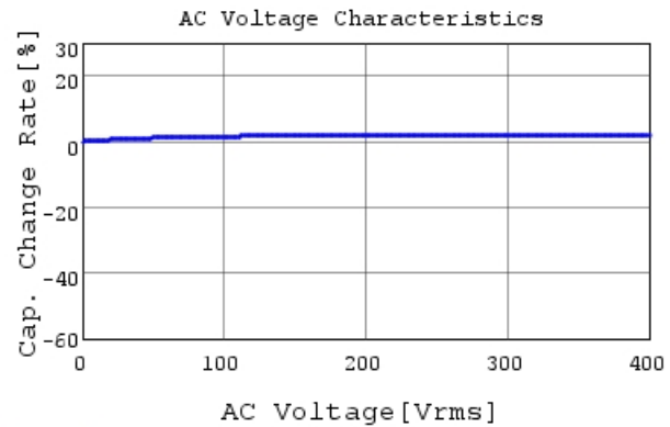
RDE7U3A101J2M1H03A C-AC Voltage capchange, I
