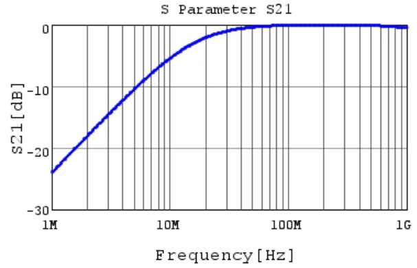
RDE7U3A101J2M1H03A S21 DCOV, 25degC
