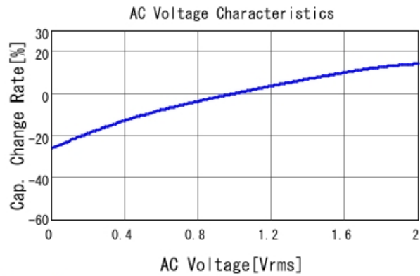
GRM31CR6YA106MA12 C-AC Voltage capchange, DCOV, 25
