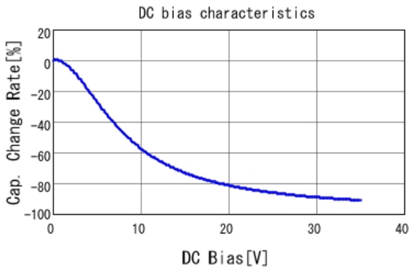
GRM31CR6YA106MA12 C-DC bias capchange, 25.0degC, A
