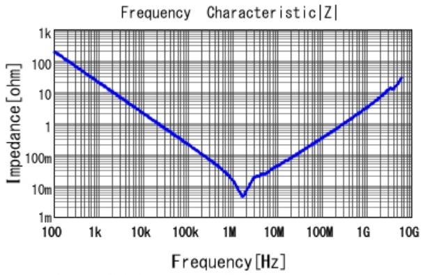
GRM31CR6YA106MA12 |Z| DCOV, 25degC
