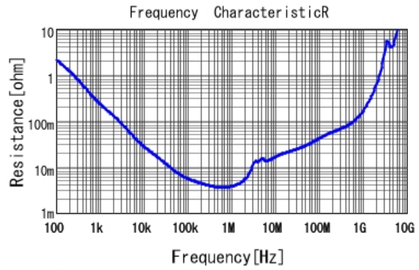
GRM31CR6YA106MA12 R DCOV, 25degC
