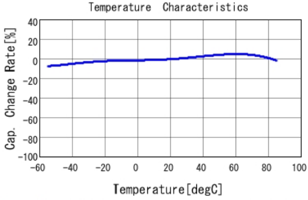
GRM31CR6YA106MA12 C-Temp. capchange, DCO. 0V, AC1. C
