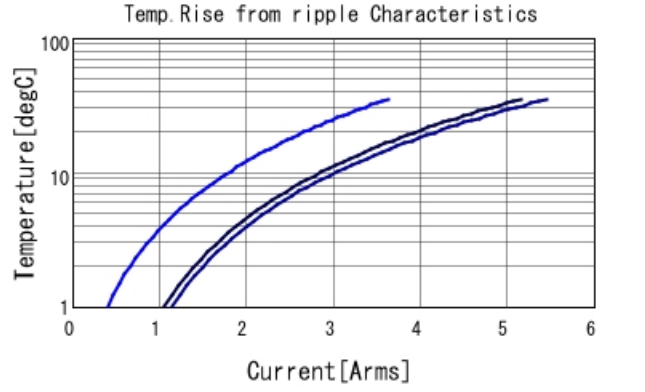
GRM31CR6YA106MA12 Temp. rise — 80kHz — 400kHz
