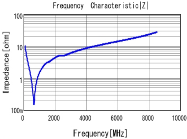
■ GRM1555C1H151JA01 |Z| DC0V, 25degC
