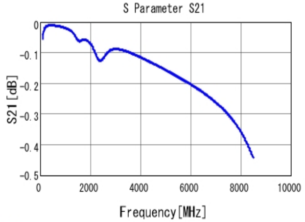
■ GRM1555C1H151JA01 S21 DCOV, 25degC
