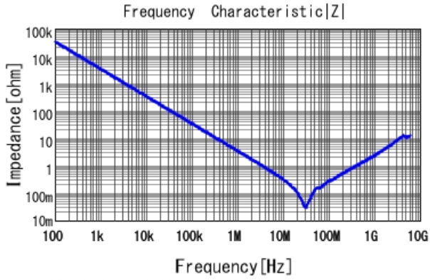
GRM21BR72A473KA01 |Z| DCOV, 25degC
