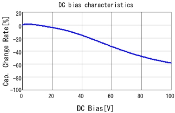
GRM21BR72A473KA01 C-DC bias capchange, 25.0degC, A
