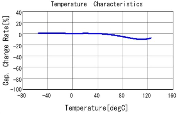
GRM21BR72A473KA01 C-Temp. capchange, DC0.0V, AC1.C
