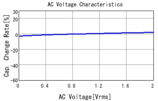
GRM21BR72A473KA01 C-AC Voltage capchange, DCOV, 25
