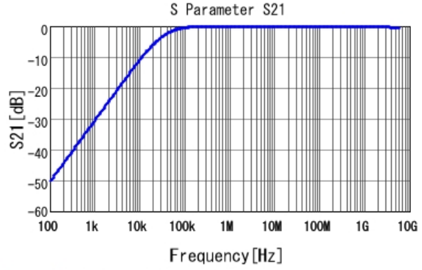
GRM21BR72A473KA01 S21 DC0V, 25degC
