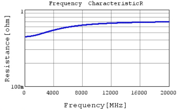
GRM0225C1E1R1CA03 R DCOV, 25degC
