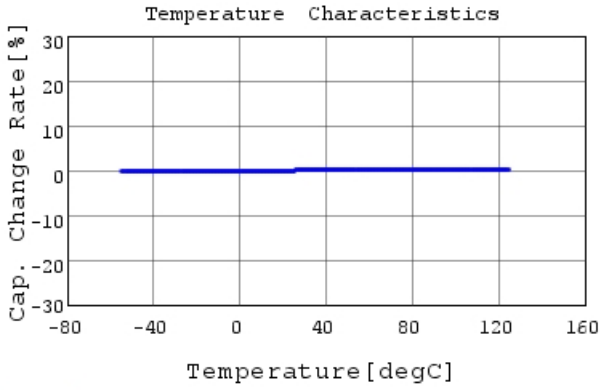
GRM0225C1E1R1CA03 C-Temp. capchange, DCOV, 1
