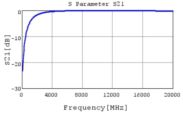
GRM0225C1E1R1CA03 S21 DCOV, 25degC
