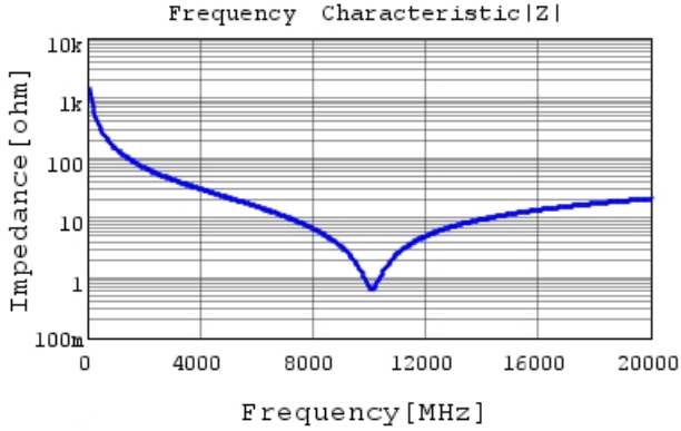
GRM0225C1E1R1CA03 |Z| DCOV, 25degC
