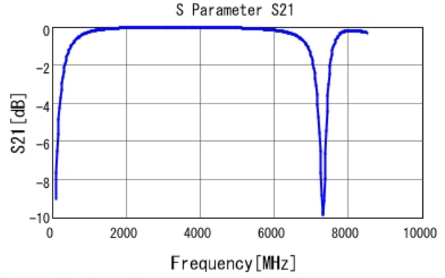
GQM1875C2E6R0CB12 S21 DCOV, 25degC
