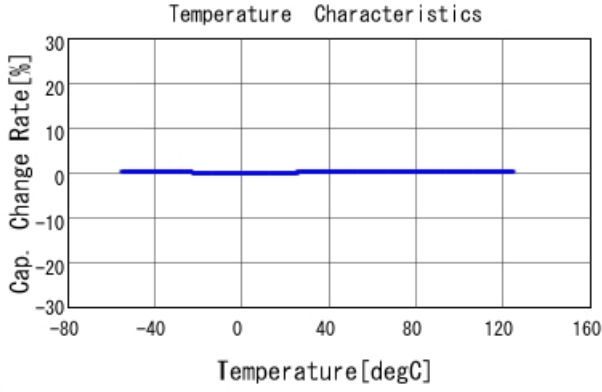
GQM1875C2E6R0CB12 C-Temp. capchange, DCOV, AC1Vrms
