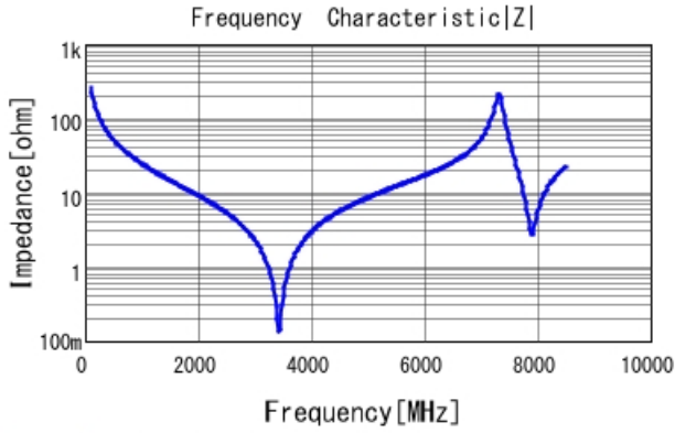
GQM1875C2E6R0CB12 |Z| DCOV, 25degC
