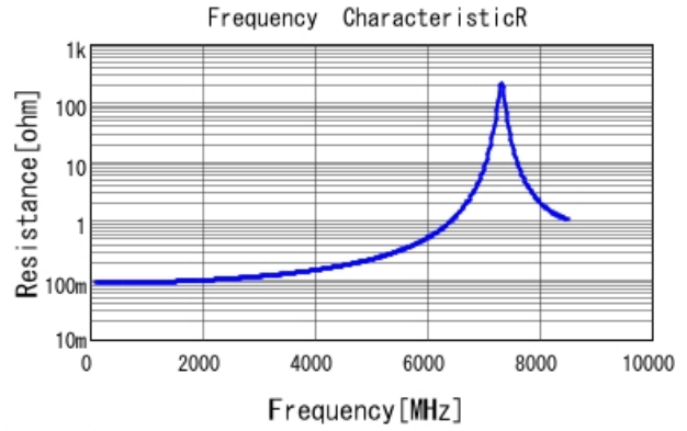
GQM1875C2E6R0CB12 R DCOV, 25degC
