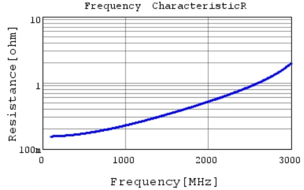
GRM31A5C2J470FW01 R DC0V, 25degC
