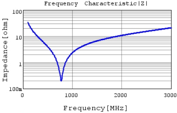
GRM31A5C2J470FW01 |Z| DC0V, 25degC
