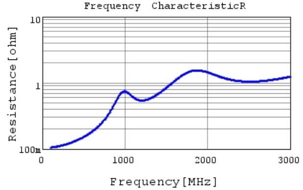
GRM31A5C2J331GW01 R DCOV, 25degC
