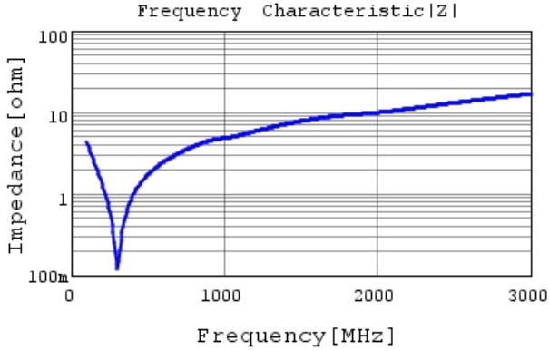
GRM31A5C2J331GW01 |Z| DCOV, 25degC
