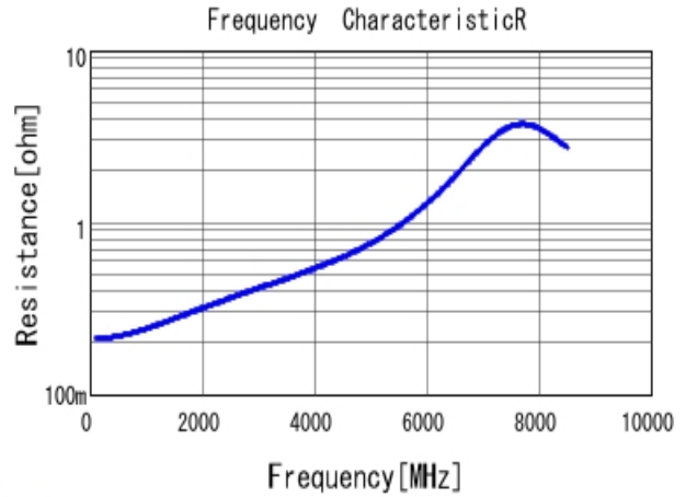
■ GRM1555C1H6R0CA01 R DCOV, 25degC
