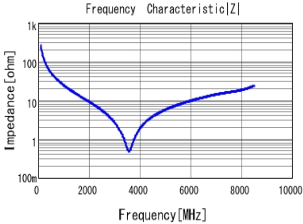
■ GRM1555C1H6R0CA01 |Z| DCOV, 25degC
