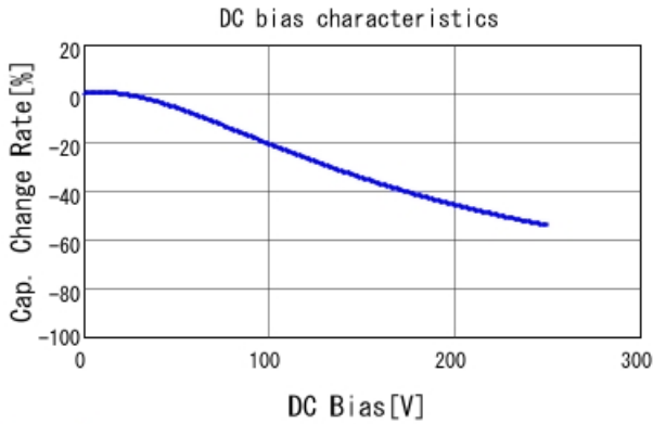
GR331AD72E333KW01 C-DC bias capchange, 25.0degC, A
