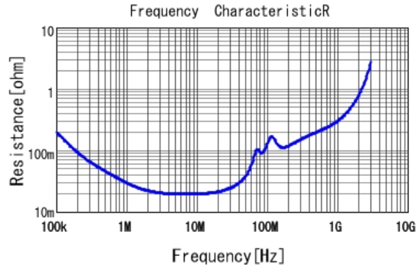
GR331AD72E333KW01 R DCOV, 25degC
