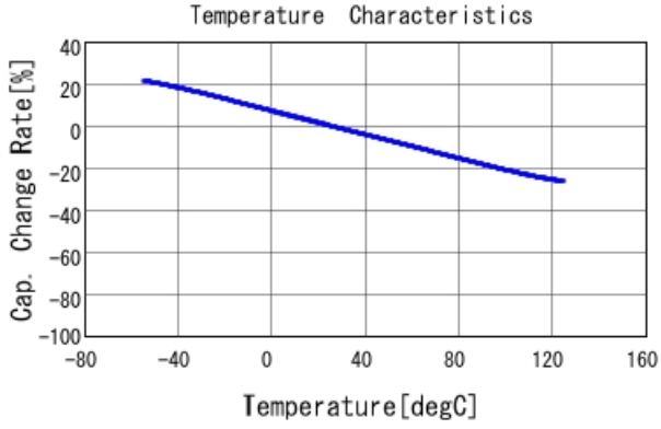
GR331AD72E333KW01 C-Temp. capchange, DCOV, AC1Vrms
