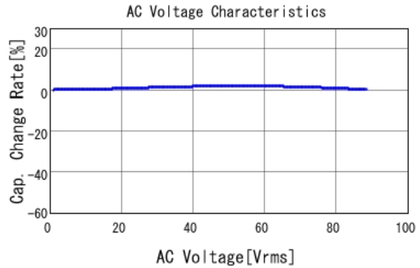
GR331AD72E333KW01 C-AC Voltage capchange, DCOV, 25
