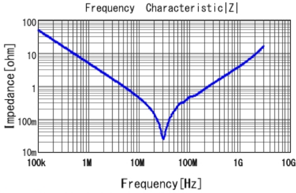
GR331AD72E333KW01 |Z| DCOV, 25degC
