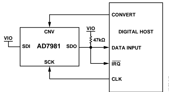
Figure 43. 3-Wire \overline{\text{CS}} Mode with Busy Indicator Connection Diagram (SDI High)
