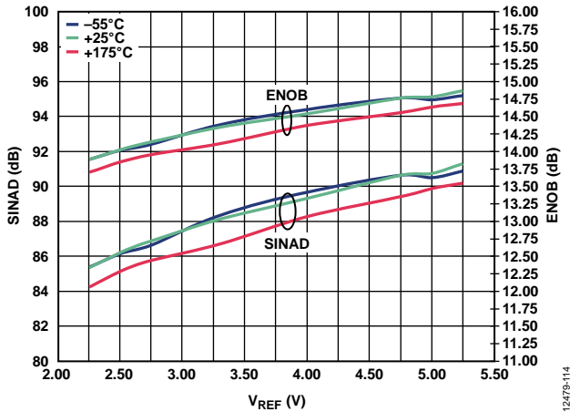
Figure 18. SINAD and ENOB vs. Reference Voltage ( V_{REF} ), MSOP
