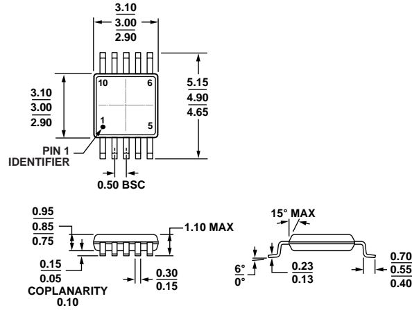
COMPLIANT TO JEDEC STANDARDS MO-187-BA Figure 56. 10-Lead Mini Small Outline Package [MSOP] (RM-10) Dimensions shown in millimeters
