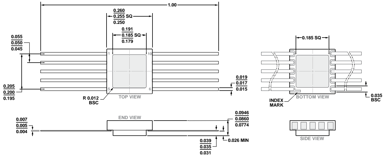
Figure 57. 10-Lead Ceramic Flat Package [FLATPACK] (F-10-2) Dimensions shown in inches
