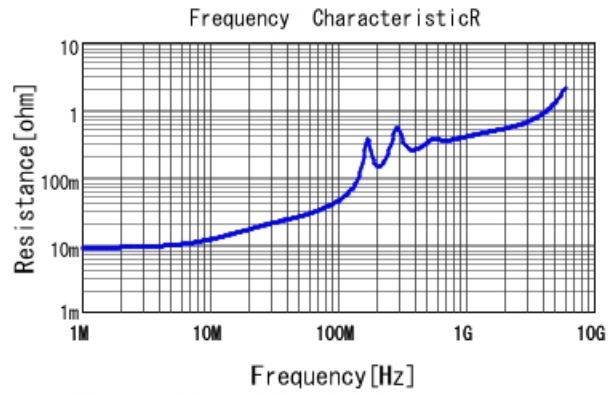
GCM3195C1H472JA16 R DCOV, 25degC
