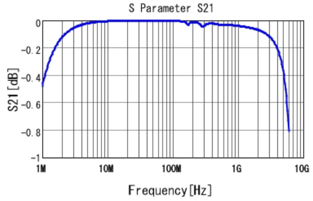
GCM3195C1H472JA16 S21 DCOV, 25degC
