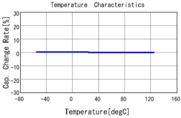
GCM3195C1H472JA16 C-Temp. capchange, DCOV, AC1Vrms
