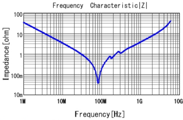
GCM3195C1H472JA16 |Z| DCOV, 25degC
