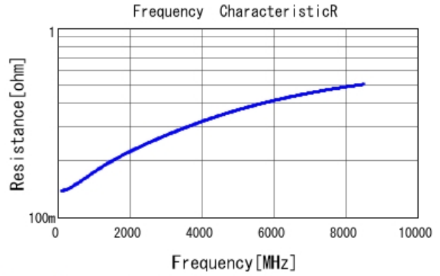
GRM0225C1E7R7DA03 R DCOV, 25degC
