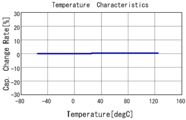
GRM0225C1E7R7DA03 C-Temp. capchange, DC0V, AC1Vrms
