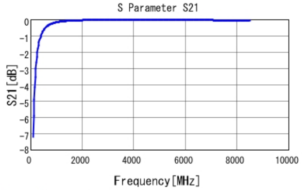
GRM0225C1E7R7DA03 S21 DC0V, 25degC
