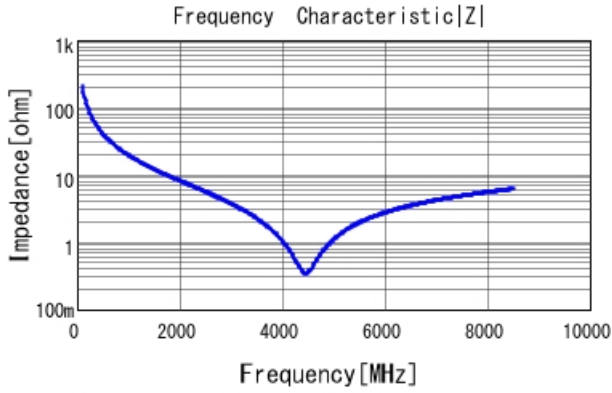
GRM0225C1E7R7DA03 |Z| DCOV, 25degC
