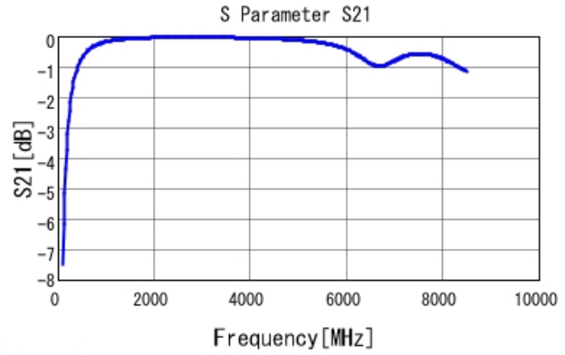
GRM1555C2A7R4CA01 S21 DCOV, 25degC
