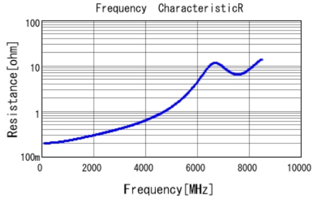
GRM1555C2A7R4CA01 R DCOV, 25degC
