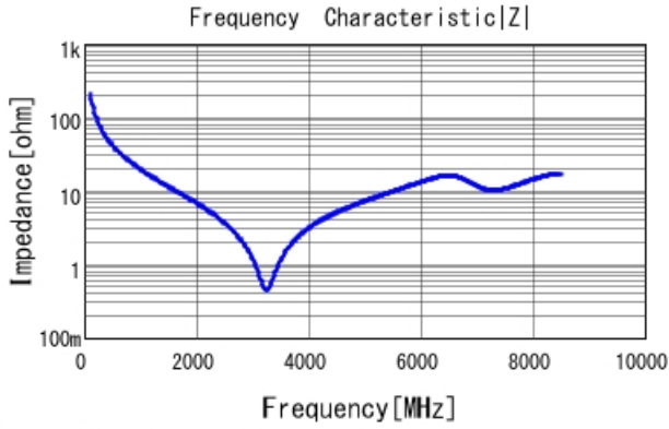
GRM1555C2A7R4CA01 |Z| DCOV, 25degC
