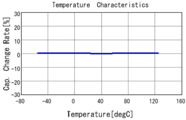
GRM1555C2A7R4CA01 C-Temp. capchange, DCOV, AC1Vrms
