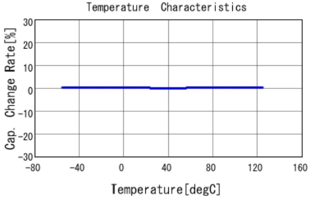
GRM1555C2A4R8CA01 C-Temp. capchange, DC0V, AC1Vrms
