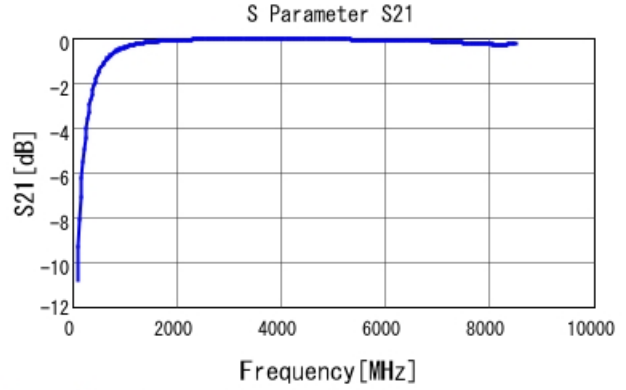
GRM1555C2A4R8CA01 S21 DC0V, 25degC
