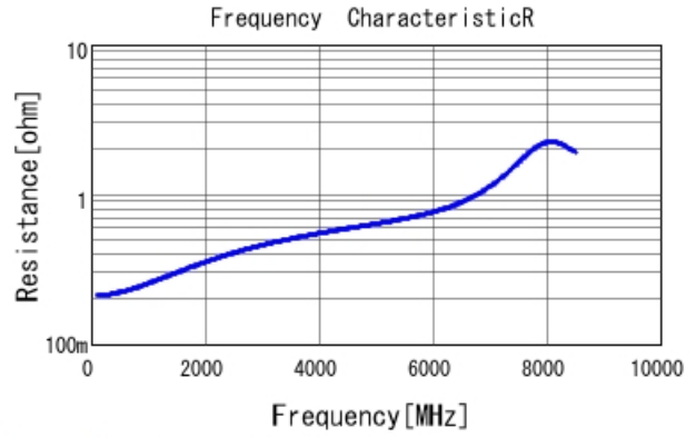
GRM1555C2A4R8CA01 R DCOV, 25degC
