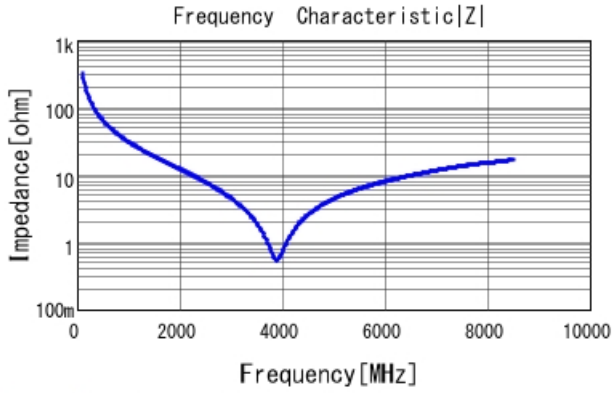
GRM1555C2A4R8CA01 |Z| DCOV, 25degC
