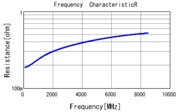
GRM0225C1E3R7CA03 R DCOV, 25degC
