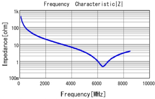
GRM0225C1E3R7CA03 |Z| DCOV, 25degC
