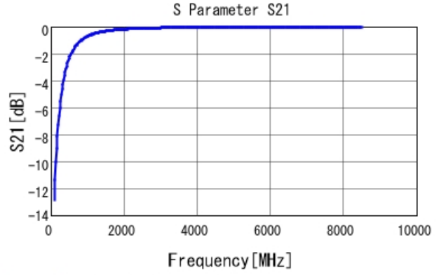
GRM0225C1E3R7CA03 S21 DC0V, 25degC
