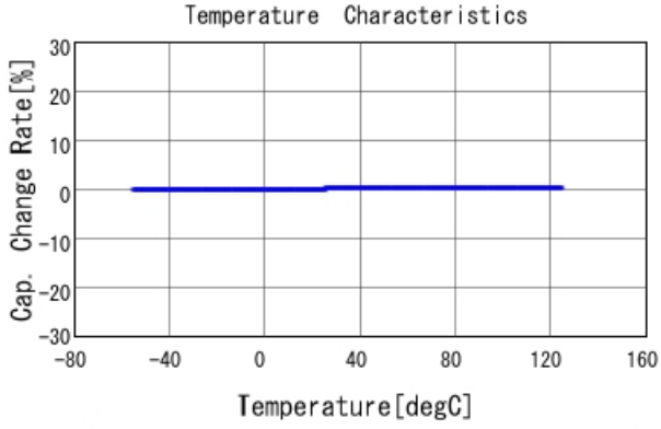
GRM0225C1E3R7CA03 C-Temp. capchange, DC0V, AC1Vrms
