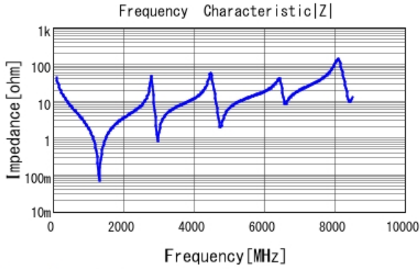
GQM2195G2E360JB12 |Z| DCOV, 25degC
