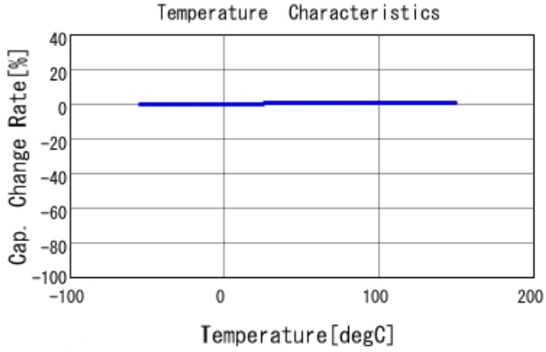
GQM2195G2E360JB12 C-Temp. capchange, DCOV, AC1Vrms
