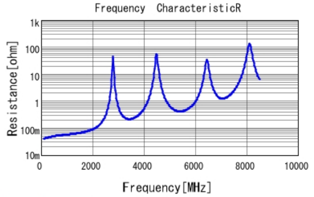
GQM2195G2E360JB12 R DCOV, 25degC
