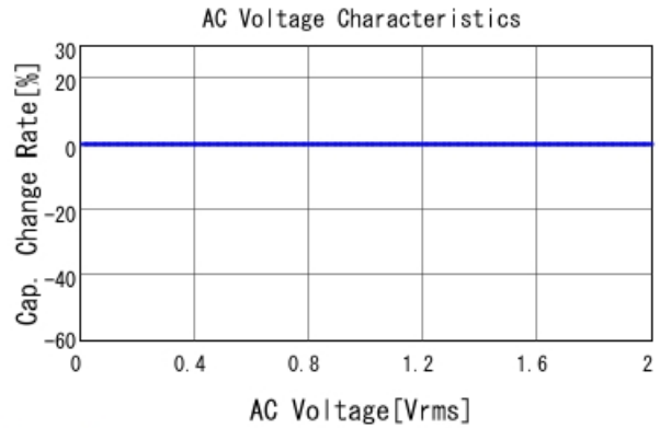
GQM2195G2E360JB12 C-AC Voltage capchange, DCOV, 25
