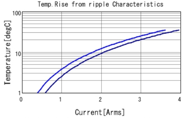
GRM188B31C225KE14 Temp. rise — 500kHz — 1MHz
