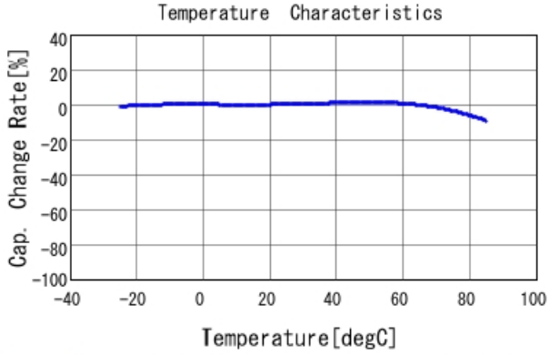
GRM188B31C225KE14 C-Temp. capchange, DC0.0V, AC0.5
