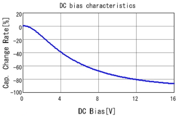
GRM188B31C225KE14 C-DC bias capchange, 20.0degC, A
