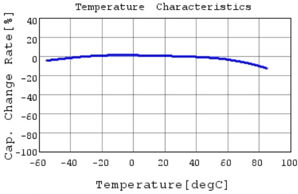
GRM022R60G473ME15 C-Temp. capchange, DC0.0V,
