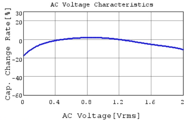
GRM022R60G473ME15 C-AC Voltage capchange, Dc
