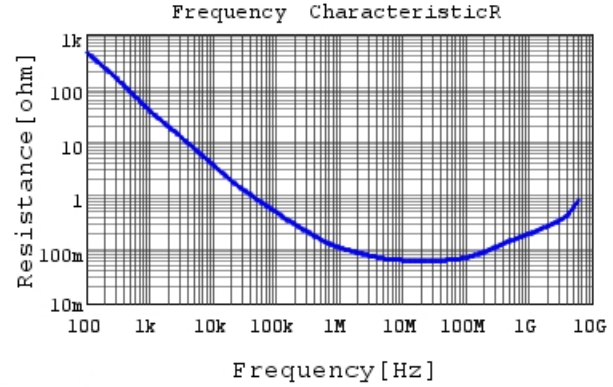
GRM022R60G473ME15 R DCOV, 25degC
