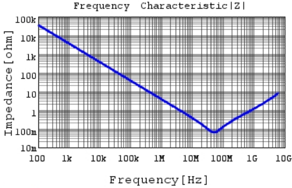
GRM022R60G473ME15 |Z| DCOV, 25degC
