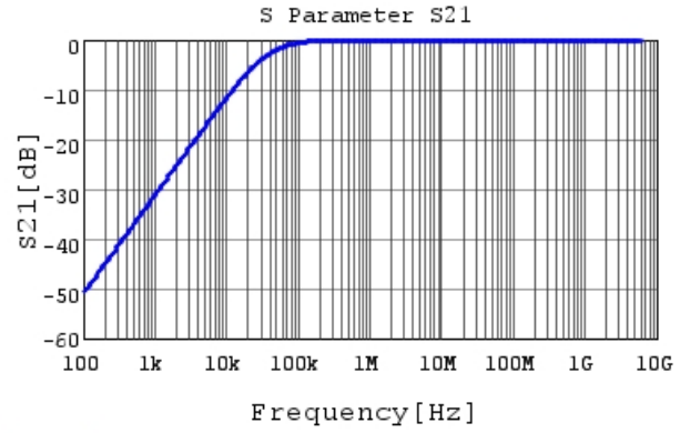
GRM022R60G473ME15 S21 DC0V,25degC
