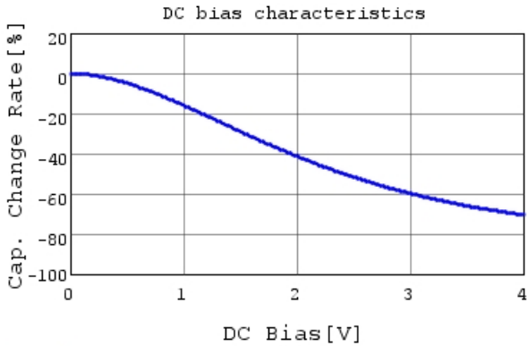
GRM022R60G473ME15 C-DC bias capchange, 25.0c
