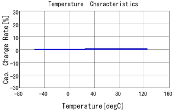
GRM0225C1E6R9CA03 C-Temp. capchange, DC0V, AC1Vrms
