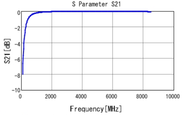
GRM0225C1E6R9CA03 S21 DC0V, 25degC
