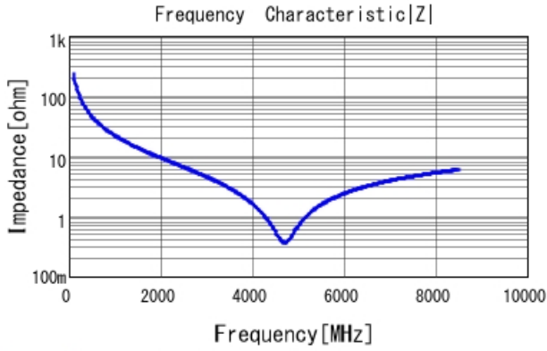
GRM0225C1E6R9CA03 |Z| DCOV, 25degC
