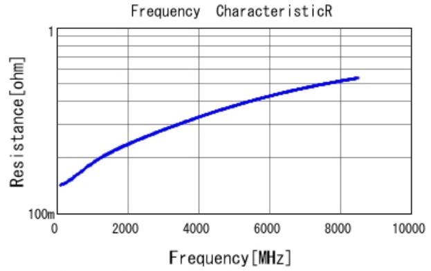
GRM0225C1E6R9CA03 R DCOV, 25degC
