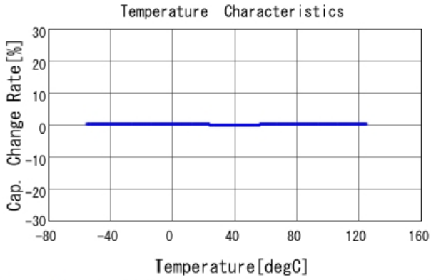
GRM1555C1H1R0BA01 C-Temp. capchange, DCOV, AC1Vrms
