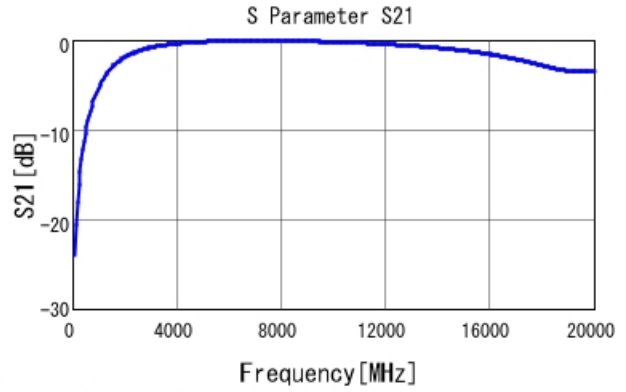
GRM1555C1H1R0BA01 S21 DCOV, 25degC
