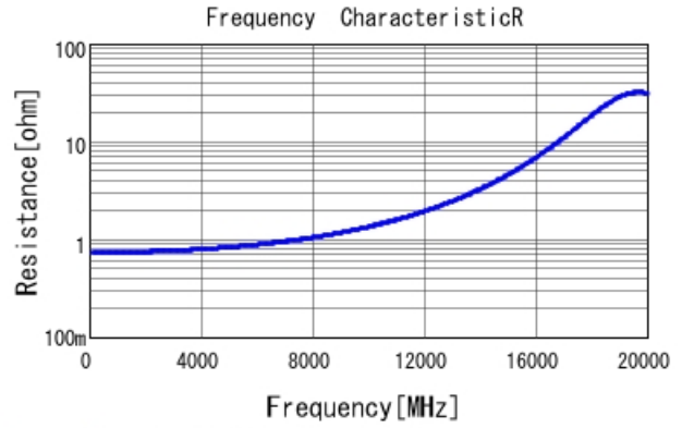
GRM1555C1H1R0BA01 R DCOV, 25degC
