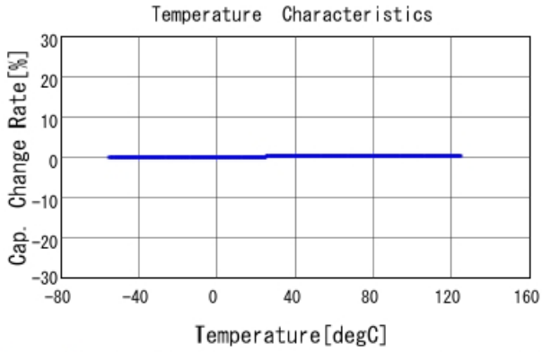
GRM1885C1H9R8CA01 C-Temp. capchange, DCOV, AC1Vrms
