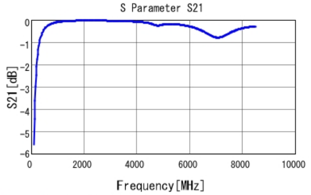
GRM1885C1H9R8CA01 S21 DCOV, 25degC
