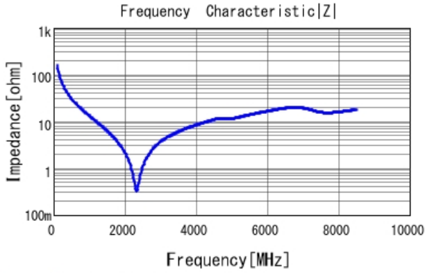
GRM1885C1H9R8CA01 |Z| DCOV, 25degC
