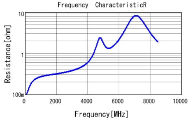
GRM1885C1H9R8CA01 R DCOV, 25degC
