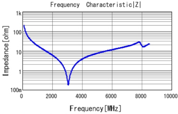
GJM1555C1H7R8WB01 |Z| DCOV, 25degC
