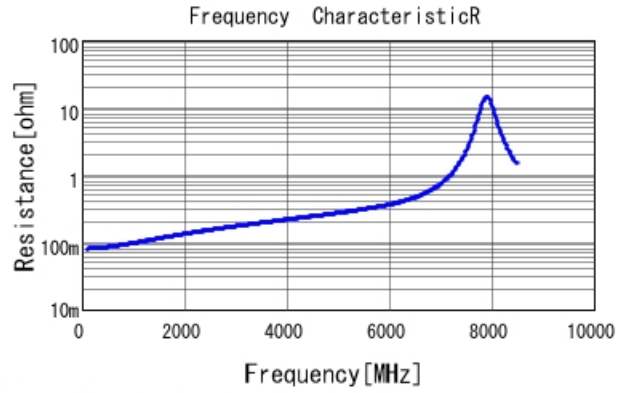
GJM1555C1H7R8WB01 R DCOV, 25degC
