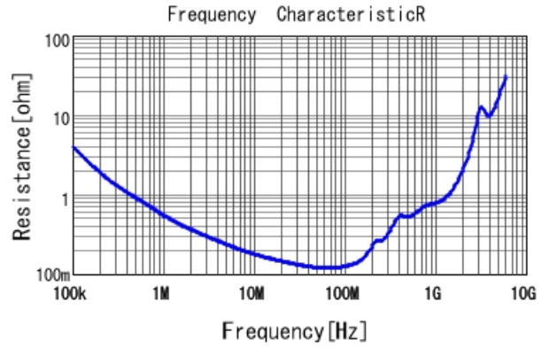
GRM31BR73A472KW01 R DCOV, 25degC
