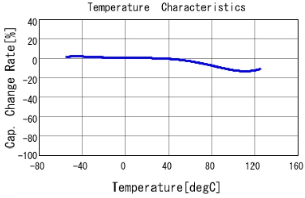
GRM31BR73A472KW01 C-Temp. capchange, DCOV, AC1Vrms
