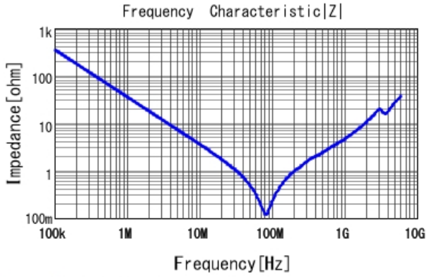
GRM31BR73A472KW01 |Z| DCOV, 25degC
