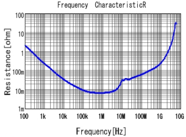
GJ431CC81E105KA01 R DC0V, 25degC
