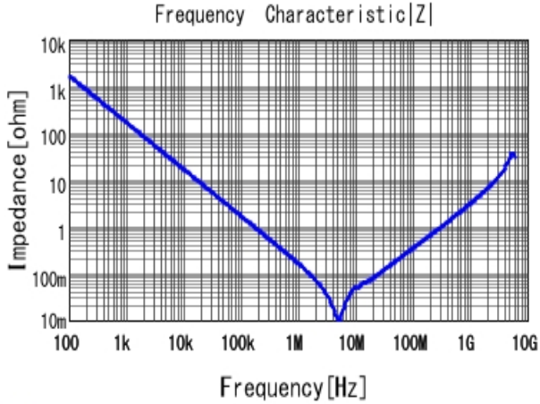
GJ431CC81E105KA01 |Z| DC0V, 25degC
