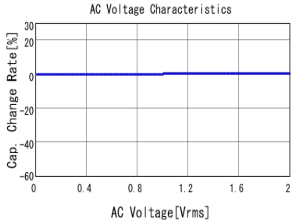
GJ431CC81E105KA01 C-AC Voltage capchange, DC0V, 25.0d
