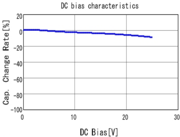
GJ431CC81E105KA01 C-DC bias capchange, 25.0degC, AC1.
