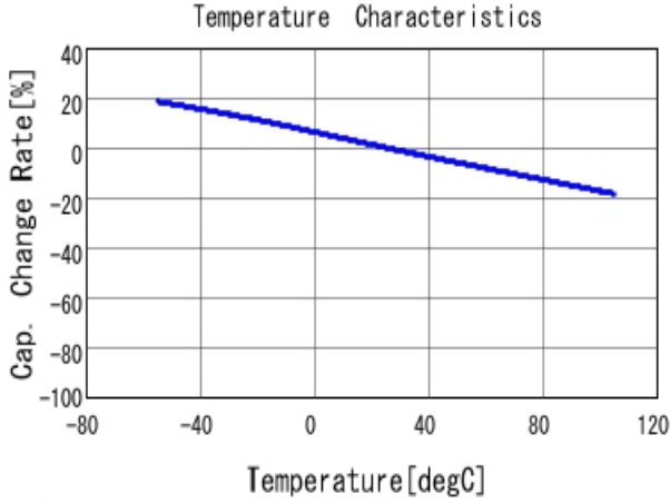
GJ431CC81E105KA01 C-Temp. capchange, DC0.0V, AC1.0V r m
