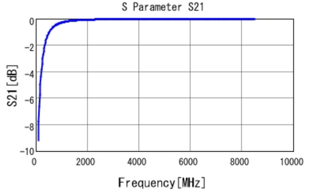
GRM0225C1E5R9DA03 S21 DC0V, 25degC
