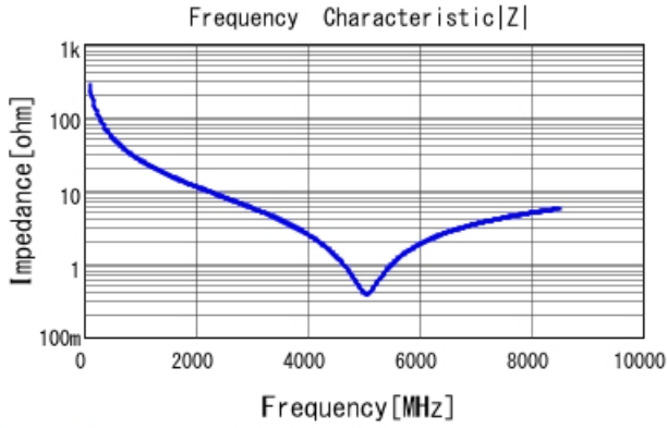
GRM0225C1E5R9DA03 |Z| DCOV, 25degC
