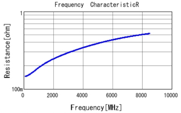
GRM0225C1E5R9DA03 R DCOV, 25degC
