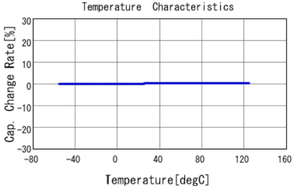
GRM0225C1E5R9DA03 C-Temp. capchange, DC0V, AC1Vrms
