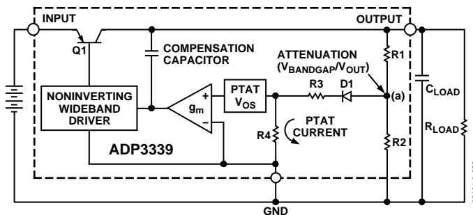
Figure 21. Functional Block Diagram
