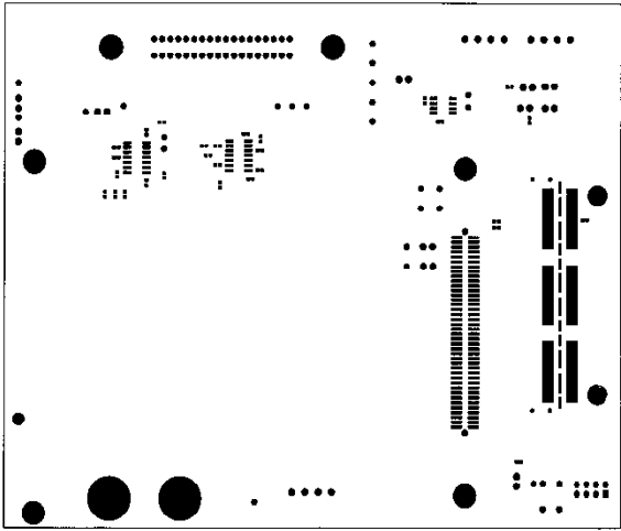
Figure 31. Top Mask
