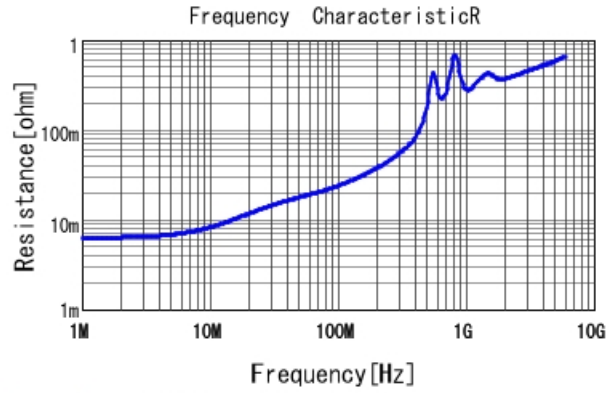
GCM1555G1H102JA16 R DCOV, 25degC
