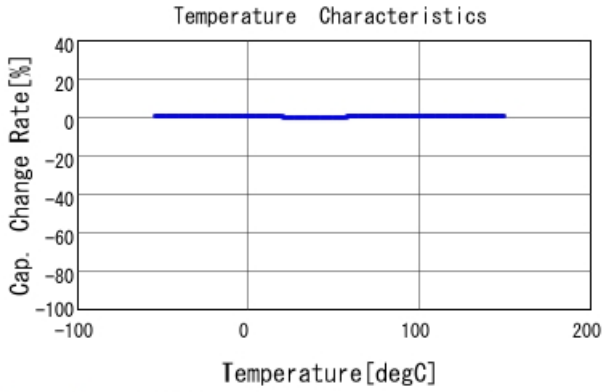
GCM1555G1H102JA16 C-Temp. capchange, DCOV, AC1Vrms
