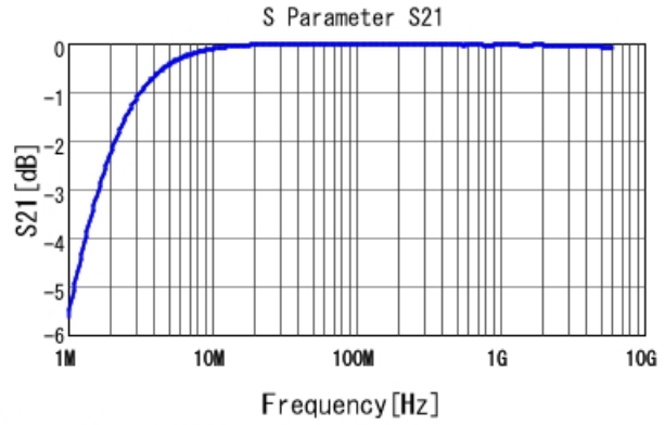
GCM1555G1H102JA16 S21 DCOV, 25degC
