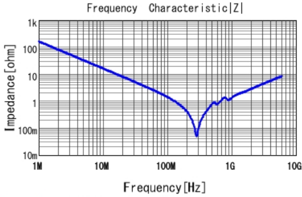
GCM1555G1H102JA16 |Z| DCOV, 25degC
