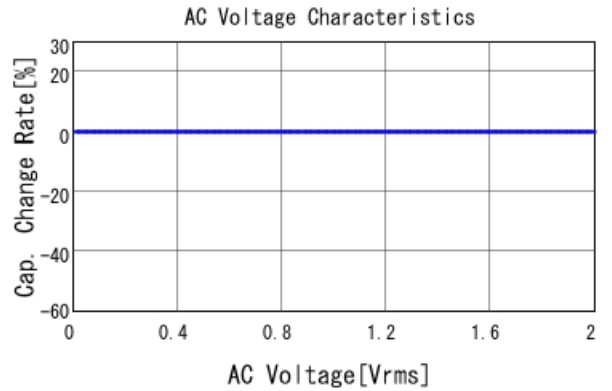
GCM1555G1H102JA16 C-AC Voltage capchange, DCOV, 25
