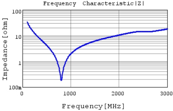
GRM31A7U3A470JW31 |Z| DC0V, 25degC
