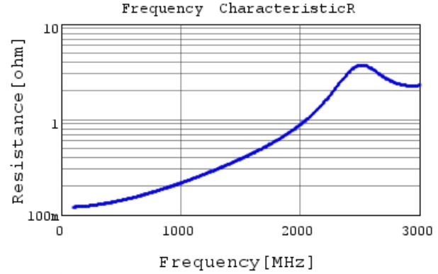
GRM31A7U3A470JW31 R DC0V, 25degC
