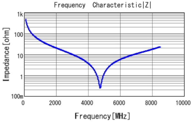
GJM1555C1H3R3WB01 |Z| DCOV, 25degC
