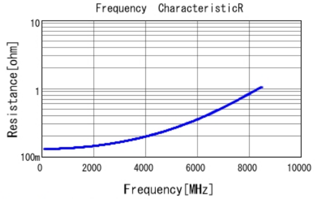
GJM1555C1H3R3WB01 R DCOV, 25degC
