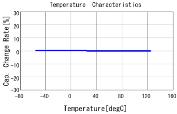
GQM1555C2D6R8BB01 C-Temp. capchange, DC0V, AC1Vrms
