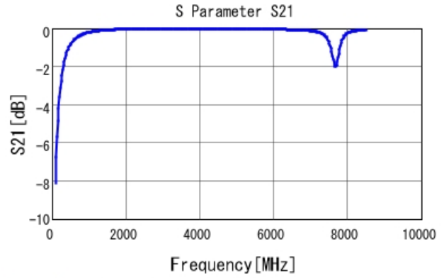
GQM1555C2D6R8BB01 S21 DC0V, 25degC
