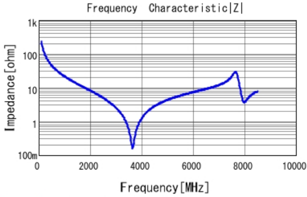
GQM1555C2D6R8BB01 |Z| DCOV, 25degC
