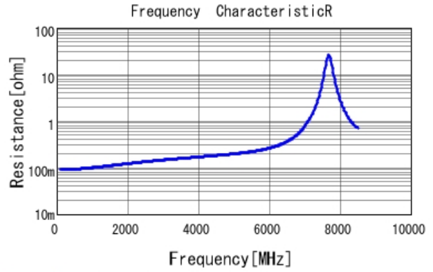
GQM1555C2D6R8BB01 R DCOV, 25degC
