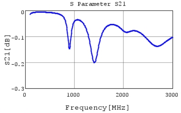
GRM21A5C2E331FW01 S21 DCOV, 25degC
