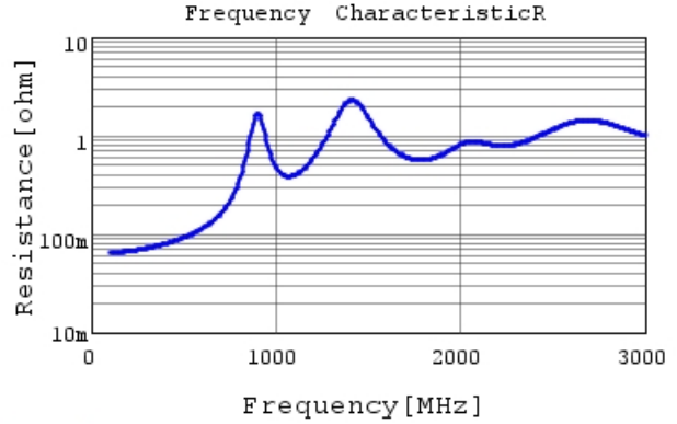
GRM21A5C2E331FW01 R DC0V, 25degC
