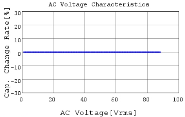
GRM21A5C2E331FW01 C-AC Voltage capchange, DC
