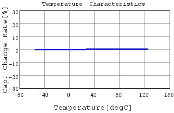
GRM21A5C2E331FW01 C-Temp. capchange, DCOV, 1
