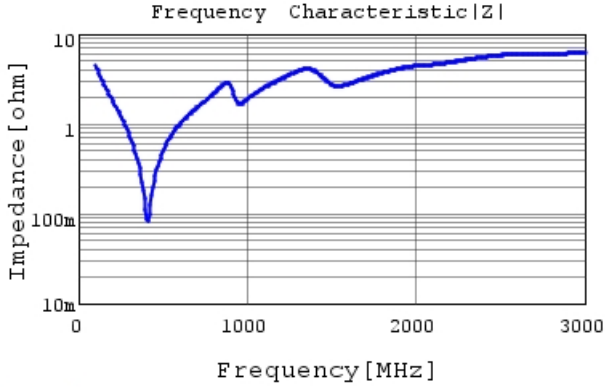
GRM21A5C2E331FW01 |Z| DC0V, 25degC
