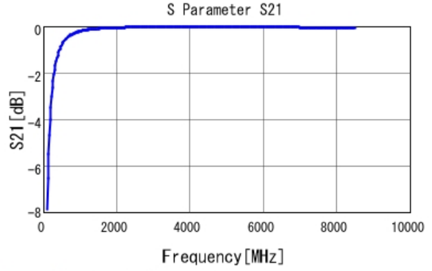
GRM0225C1E7R0DA03 S21 DCOV, 25degC
