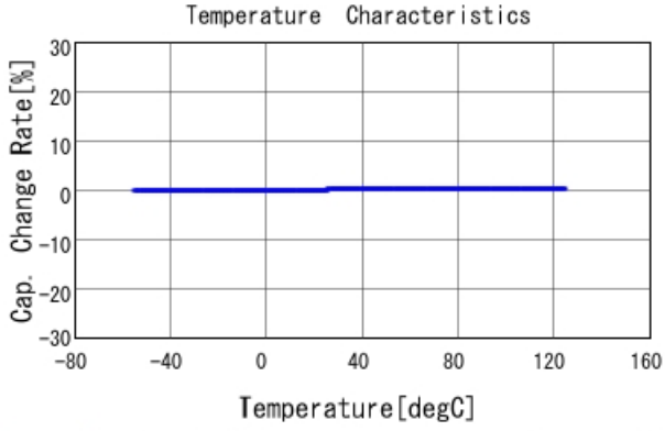
GRM0225C1E7R0DA03 C-Temp. capchange, DCOV, AC1Vrms
