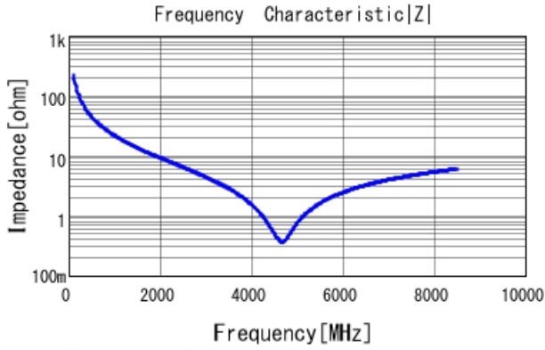
GRM0225C1E7R0DA03 |Z| DCOV, 25degC
