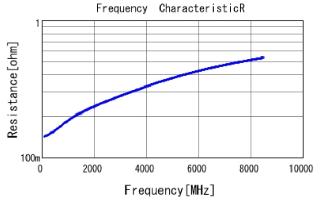
GRM0225C1E7R0DA03 R DCOV, 25degC
